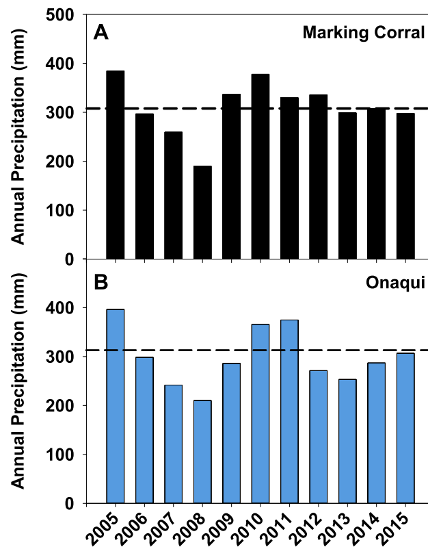
Fig. 3. Estimated annual precipitation for the Marking Corral (A) and Onaqui (B) study sites for the year prior to the study (2005) and the duration of the study period (2006–2015). The bold dashed horizontal line in each graph marks the mean annual precipitation for the respective site for years 1971–2015. Data from Prism Climate Group (2017) as estimates from a 4-km spatial grid.
